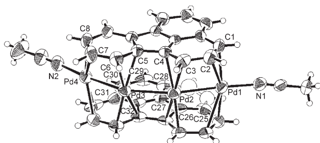
Figure 2. Molecular structure of 4a ; probability ellipsoids set at 50%; [B(Ar f ) 4 ] − counterions, and free fluoranthene and solvent molecules omitted for clarity. Selected bond lengths [Å] and angles [°]: Pd1–Pd2 2.579(1), Pd2–Pd3 2.622(1), Pd3–Pd4 2.575(2), Pd1–C1 2.21(1), Pd1–C2 2.35(1), Pd2–C3 2.16(1), Pd2–C4 2.21(1), Pd3–C5 2.26(1), Pd3–C6 2.20(1), Pd4–C7 2.57(2), Pd4–C8 2.21(1); Pd1–Pd2–Pd3 157.72(6), Pd2–Pd3–Pd4 154.67(6), N1–Pd1–Pd2 176.7(3), Pd3–Pd4–N2 173.9(4).
