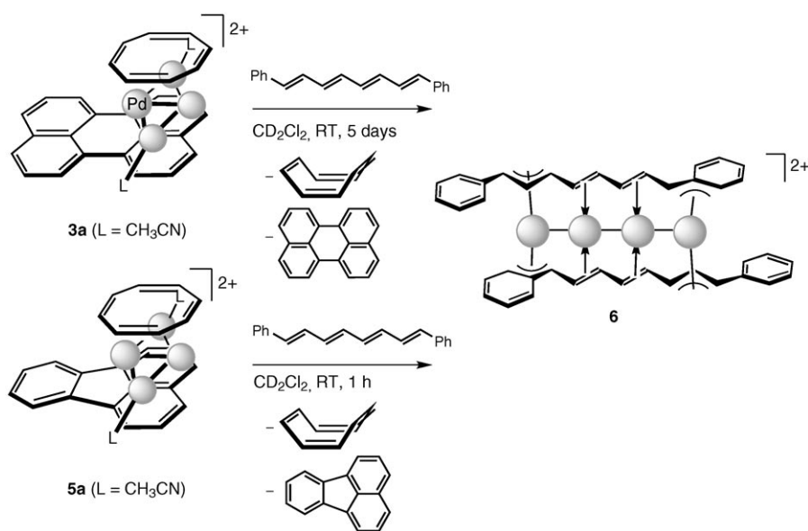
Scheme 4. Sheet-to-chain rearrangement of the Pd 4 moiety. Counterions are [B(Ar f ) 4 ] − .
