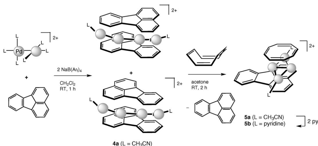
Scheme 3. Synthesis of the bis(fluoranthene) Pd 4 complex 4a (two isomers: non-eclipsed (top), eclipsed (bottom)) and fluoranthene–cot mixed sandwich Pd 4 complexes 5a and 5b . Counterions are [B(Ar f ) 4 ] − .
