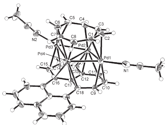
Figure 1. Molecular structure of 3a ; probability ellipsoids set at 50%; [B(Ar)_4]^- counterions and free perylene omitted for clarity. Selected bond lengths [Å] and angles [°]: Pd1–Pd2 2.749(1), Pd2–Pd3 2.711(1), Pd3–Pd4 2.757(1), Pd4–Pd1 2.715(1), Pd2–Pd4 2.874(1), Pd1–N1 2.19(1), Pd3–N2 2.19(1), Pd1–C1 2.24(1), Pd1–C2 2.21(1), Pd2–C3 2.21(1), Pd2–C4 2.19(1), Pd3–C5 2.22(1), Pd3–C6 2.21(1), Pd4–C7 2.193(10), Pd4–C8 2.188(10), Pd1–C9 2.27(1), Pd1–C10 2.25(1), Pd2–C11 2.37(1), Pd2–C12 2.172(10), Pd2–C13 2.32(1), Pd3–C14 2.29(1), Pd3–C15 2.27(1), Pd4–C16 2.404(9), Pd4–C17 2.163(9), Pd4–C18 2.346(10), C1–C2 1.41(2), C2–C3 1.45(2), C3–C4 1.41(2), C4–C5 1.45(2), C5–C6 1.41(2), C6–C7 1.45(1), C7–C8 1.42(2), C8–C1 1.42(2); Pd1–Pd2–Pd4 57.68(3), Pd4–Pd2–Pd3 59.06(3), Pd2–Pd3–Pd4 63.43(3), Pd3–Pd4–Pd2 57.51(3), Pd2–Pd4–Pd1 58.85(3).
